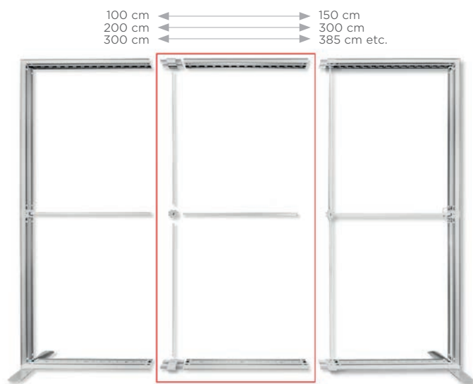
The XL Set enables to increase the LUNIX™ system width by 50, 85 or 100 cm.
