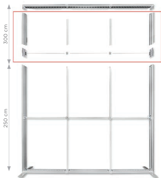
The Long Set allows to heighten the LUNIX™ by 50 cm – up to 300 cm.
