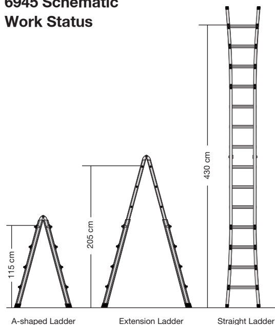
Can be quickly converted into a straight ladder, high operating convenience.
