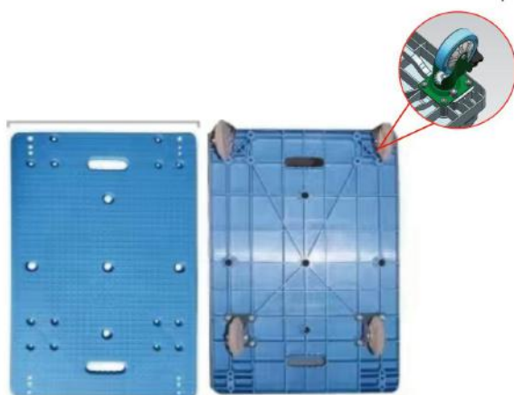
Back of the base plate
