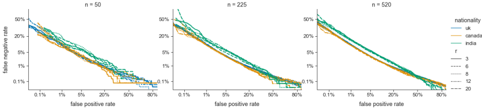
Figure 5.9: DET curves show variability in evaluation outcomes for evaluation sets with 50, 225 and 520 utterance pairs ( n ) for Canadian, Indian and UK speakers. For each n five datasets were generated with different random seeds.
