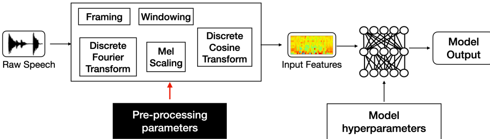
Figure 6.1: Audio processing pipeline during training and inference
