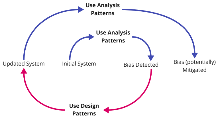
Figure 4.3: Interaction between analysis and design patterns
