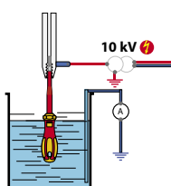
ELECTRICAL TEST (10.000V)
