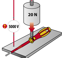
PRESSURE TEST (5000V)
