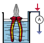
ELECTRICAL TEST (10.000V)
