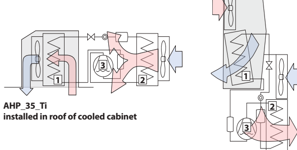
AHP_35_Ti installed on side panel of cooled cabinet
