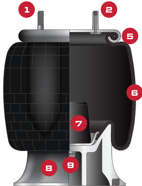
Rolling Lobe Airspring
