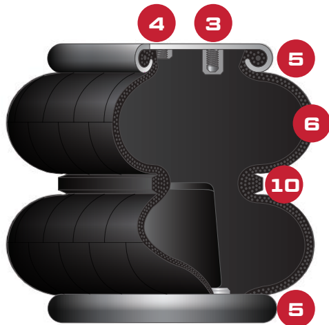
Convoluted Airspring
