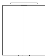
Neutron 44500 60 x 72 x 12.5(17.5)cm
