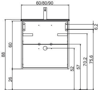
SCHEMAS TECHNIQUES
