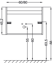
SCHEMAS TECHNIQUES
