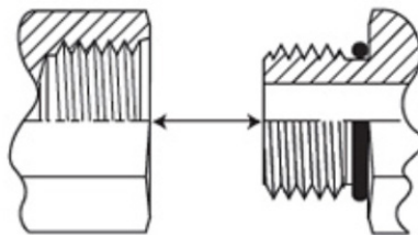
Metric Port (boss seal) (ISO 6149)
