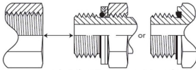
Metric Port (retained & captive seal) (ISO 9974-1 & 9974-2)
