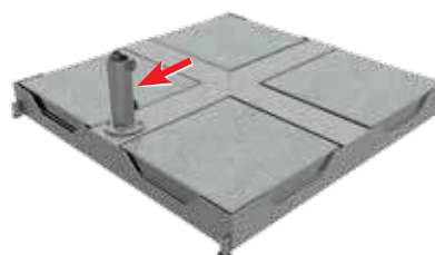
Monaco 8 Z, can be remounted for cantilever parasols
