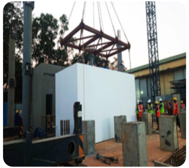
February 4 (Day 4): Prefabricated prefinished toilet pods placed in position on GF
